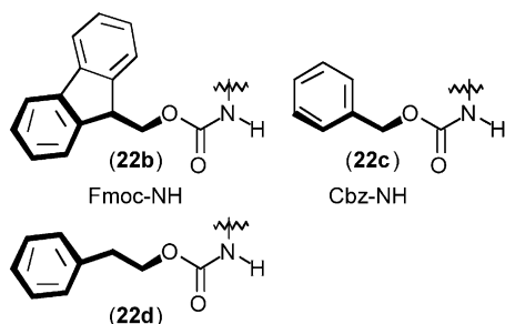
Figure 2. Comparison of N-terminal protecting groups for peptide 22 .
