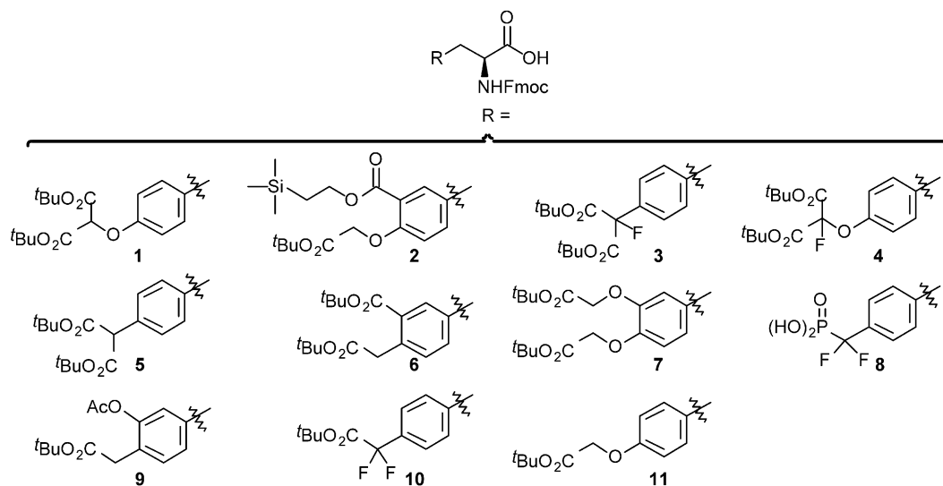
Figure 1. Structures of pTyr mimetic reagents used for solid-phase synthesis of tripeptide products.
